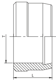
SB – Single Bite Ferrule (Single Cutting Edge)
