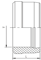
DB – Double Bite Ferrule (Double Cutting Edge)
